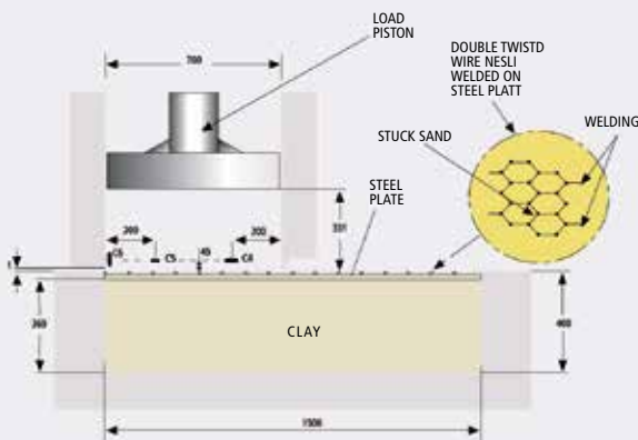
Direct smear box, testing interface soil/mesh
