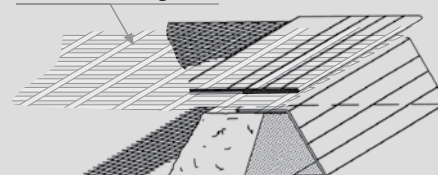
Folding of the face upper side. Placement of the next unit and attaching by stainless steel rings to the unit below. Possible layer of Geogrids.
