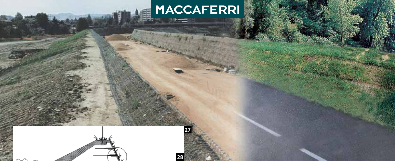
27-28. Green Terramesh® sound barrier in urban area, Bologna-Italy.
