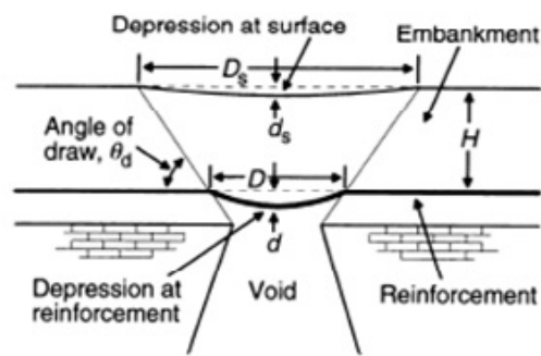
Figure 74 — Parameters used to determine reinforcement
